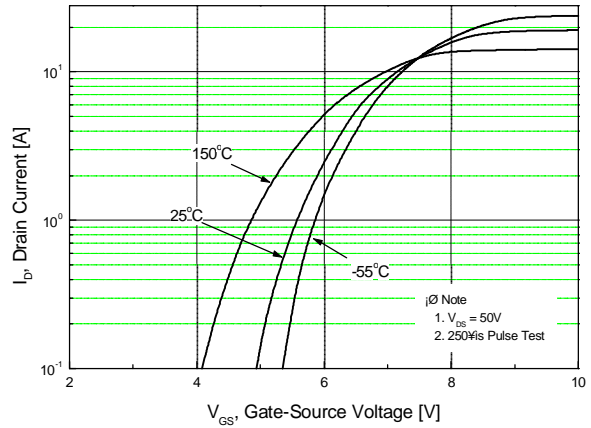
Fig 2. Transfer Characteristics
