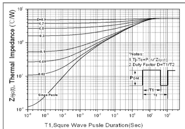
Fig.8. Transient thermal response curve(TO-220FT)
