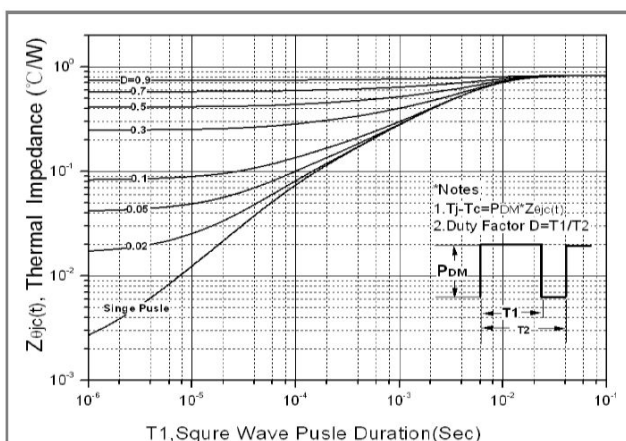
Fig.10. Transient thermal response curve(IPAK)
