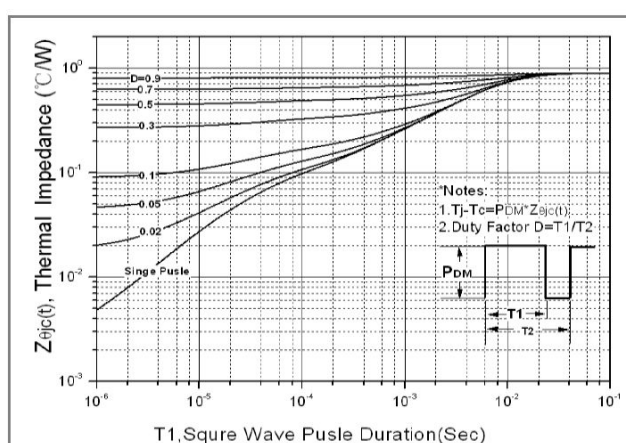
Fig.12. Transient thermal response curve(DPAK)
