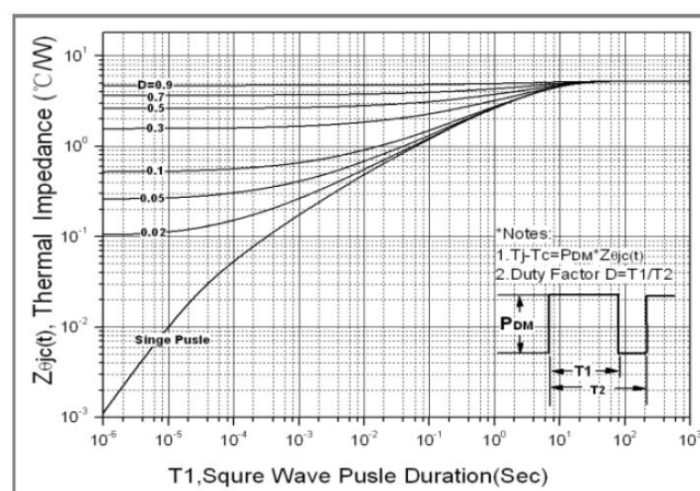
Fig.8. Transient thermal response curve(TO-220FT)
