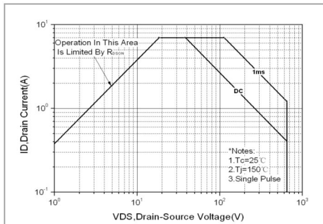
Fig.13. Maximum safe operating area(DPAK)
