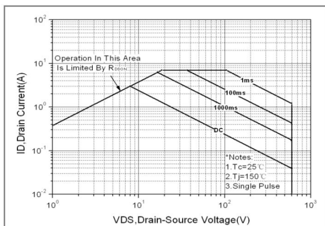
Fig.9. Maximum safe operating area(TO-220C)
