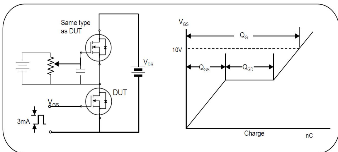
Fig.16. Gate charge test circuit & waveform
