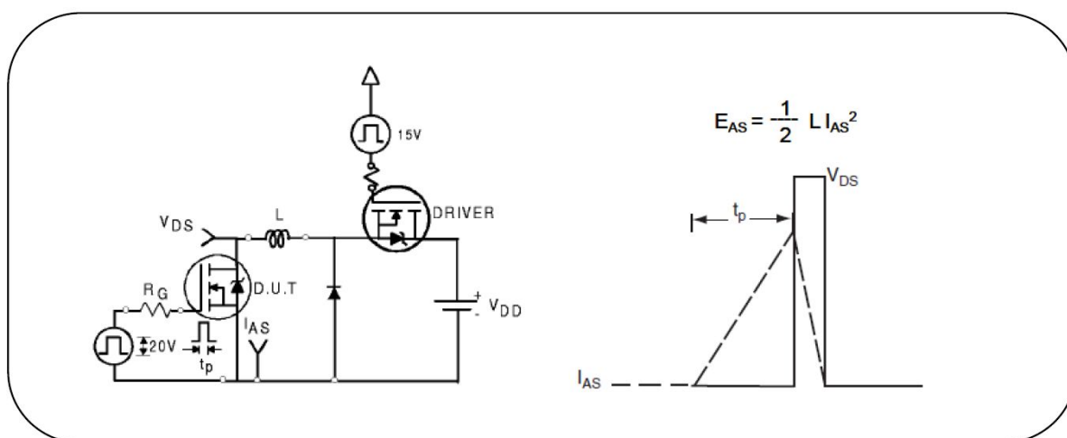
Fig.18. Unclamped inductive switching test circuit & waveform
