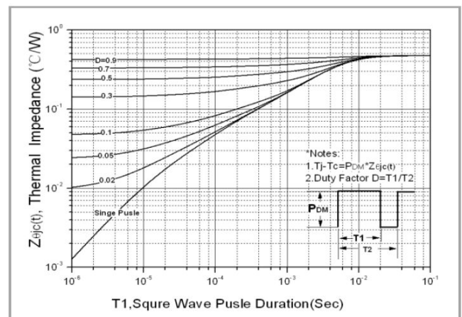
Fig.14. Transient thermal response curve(DPAK)
