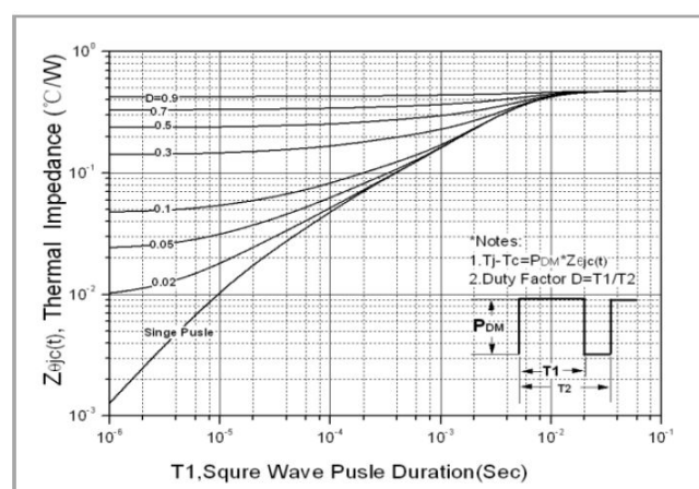
Fig.10. Transient thermal response curve(TO-220C)
