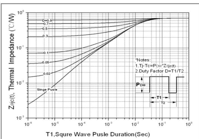
Fig.12. Transient thermal response curve(IPAK)
