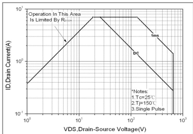
Fig.11. Maximum safe operating area(IPAK)
