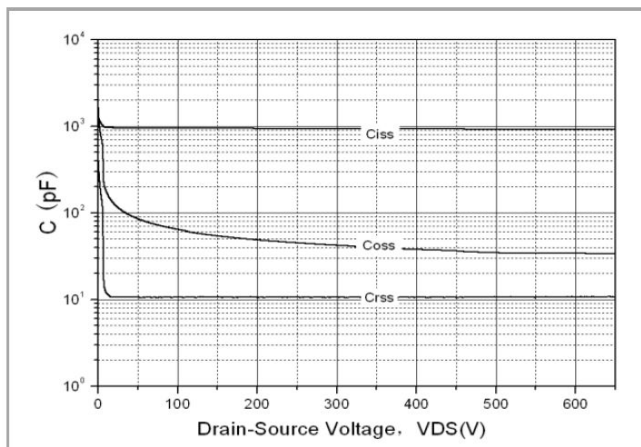
Fig.9. Capacitance characteristics
