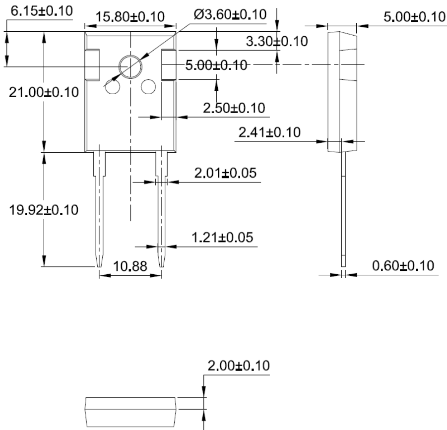
Fig8. Package Outline
