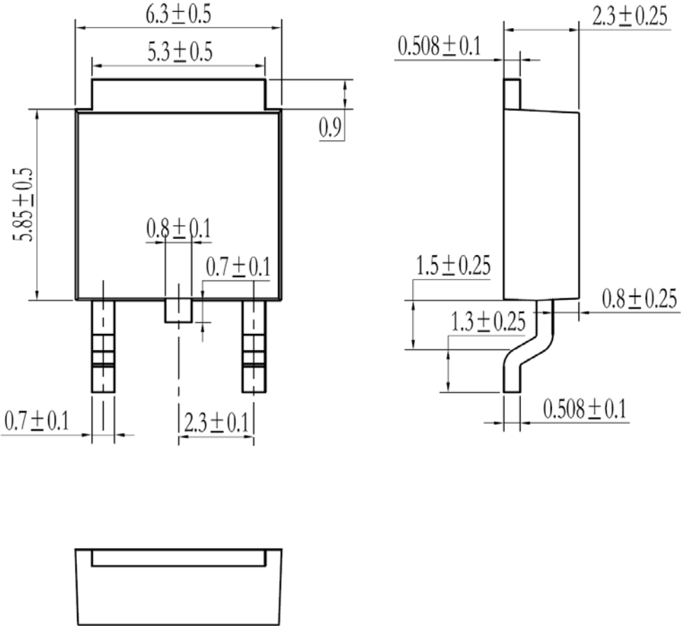
Dimensions in Millimeters Fig8. Package Outline
