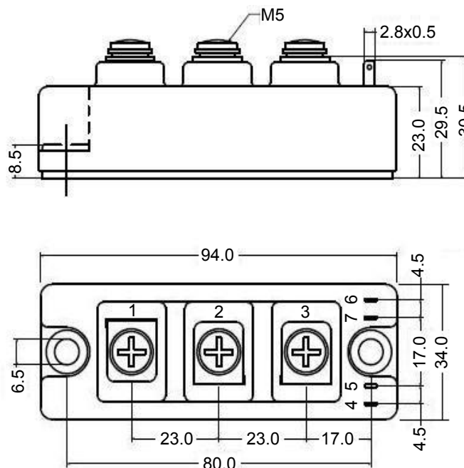
Dimensions in mm Figure16. Package Outlines
