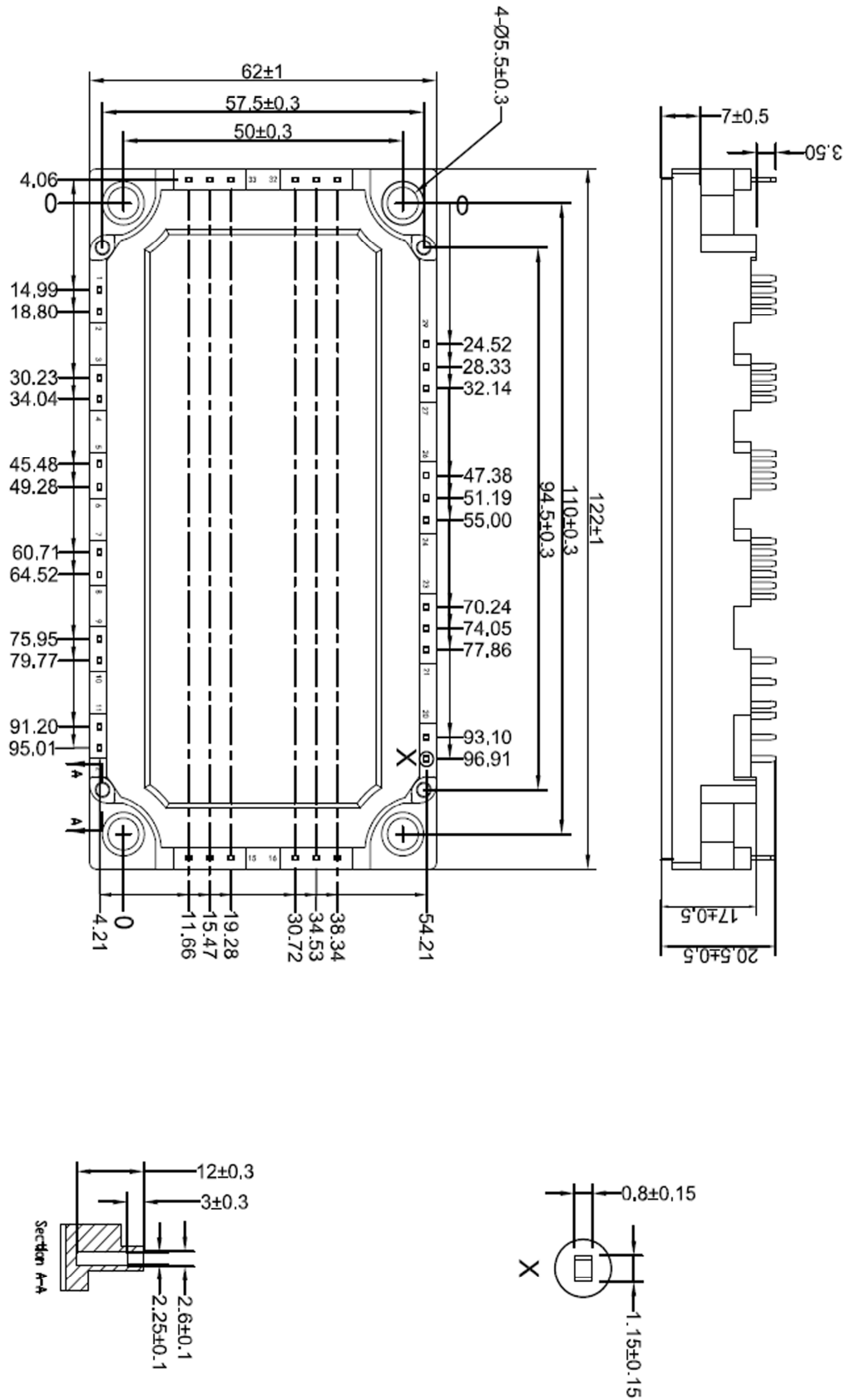
Dimensions in (mm) Figure 15. Package Outline
