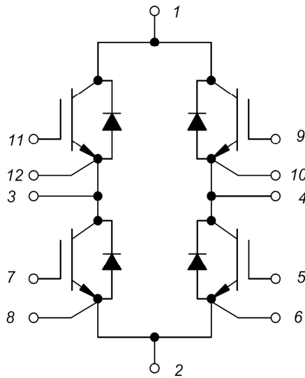
Figure 13. Circuit Diagram
