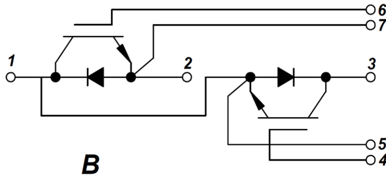
Figure 13. Circuit Diagram
