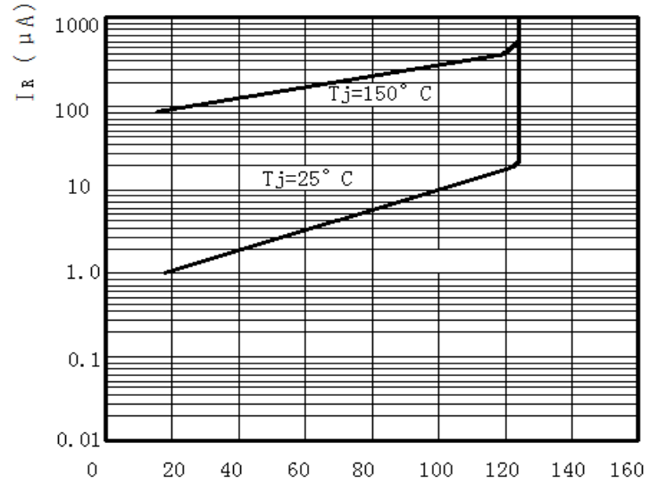
FIGURE 2. REVERSE CURRENT vs REVERSE VOLTAGE
