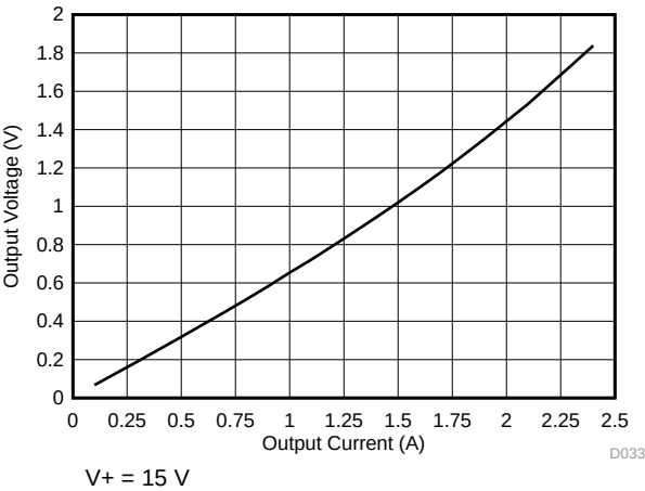
图 9. Output Swing from GND vs Output Current (Sinking)
