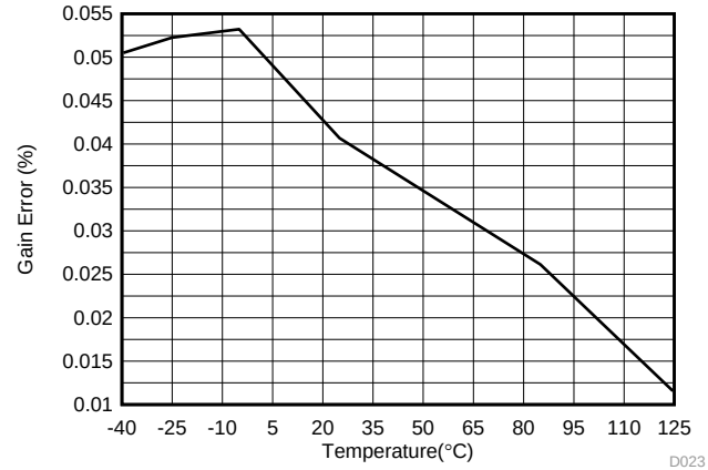
图 14. Gain Error vs Temperature
