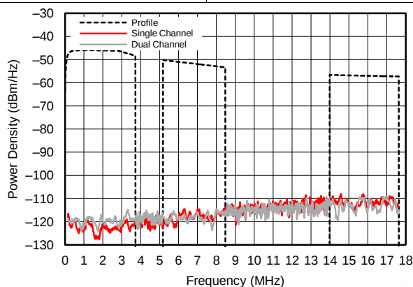
Figure 35. ADSL MTPR
