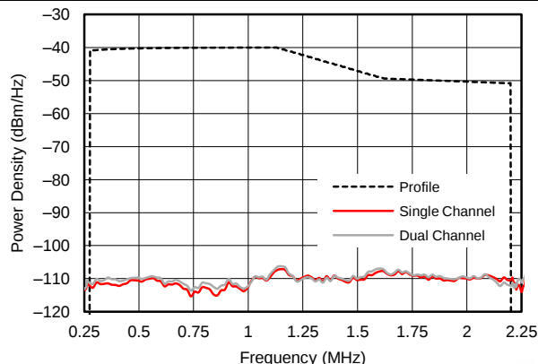
Figure 35. ADSL MTPR
