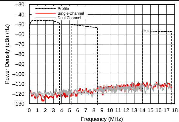
Figure 11. Profile 8 MTPR
