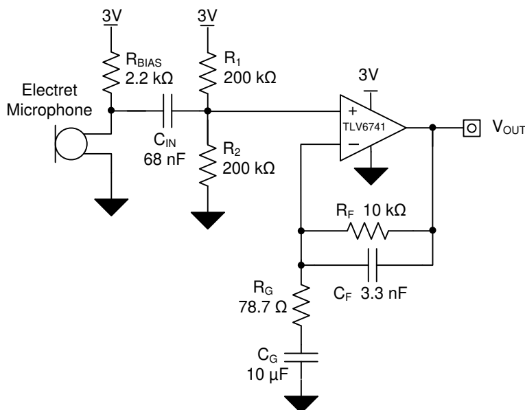
Figure 85. Microphone Preamplifier
